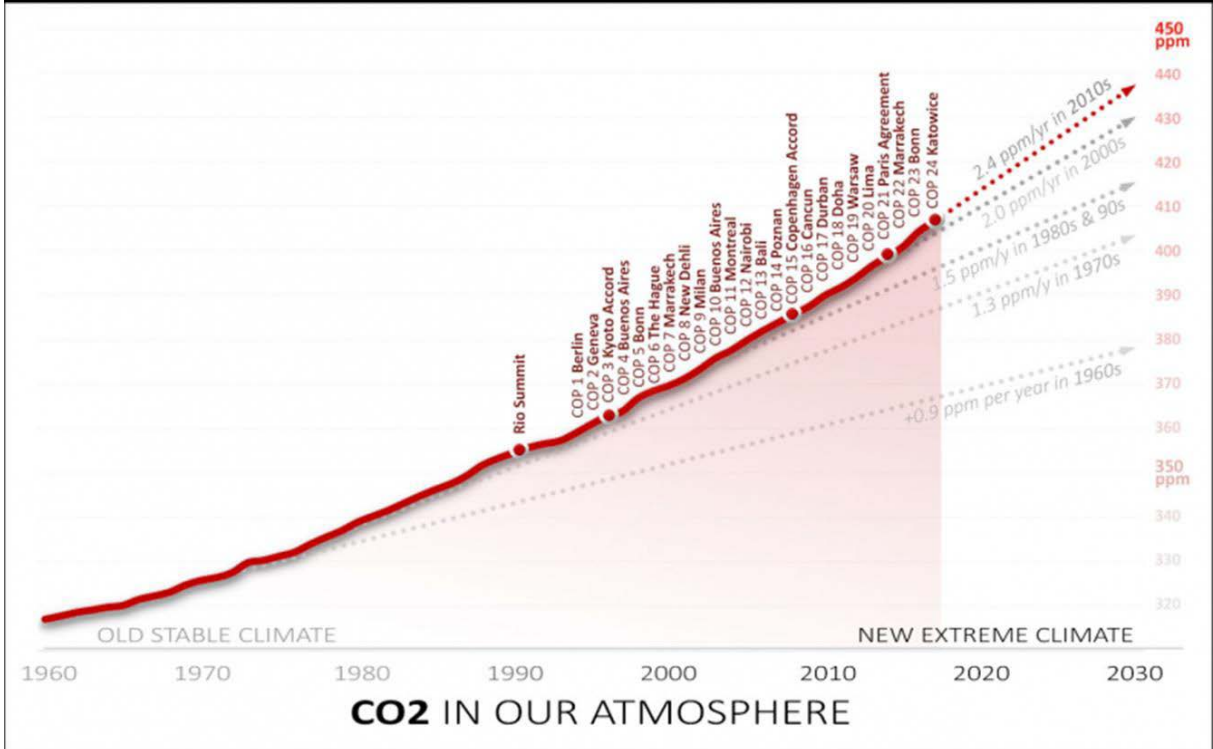
TOTAL CO2 IN OUR ATMOSPHERE -- Data from NOAA ESRL showing part-per-million (ppm) increases per year at www.esrl.noaa.gov/gmd/ccgg/trends/ . Decade trends lines show the average annual CO2 increase for that decade, continued out to 2030. Chart by Barry Saxifrage at NationalObserver.com and VisualCarbon.org. Dec 2018.
